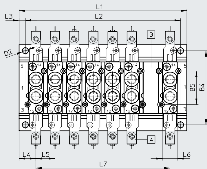
[1] Manifold block
