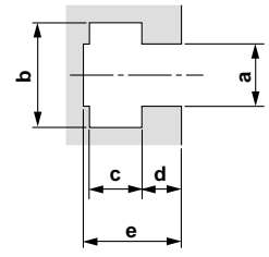
T-slot dimensions
