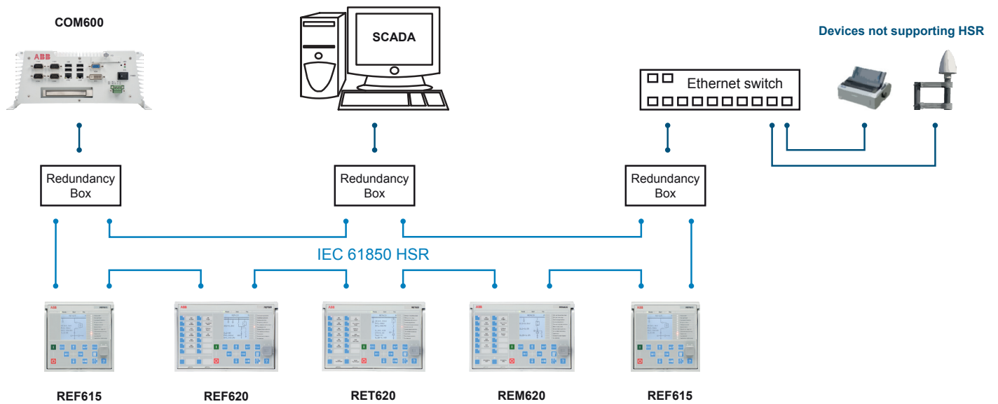
Figure 8. High availability seamless redundancy (HSR) solution
