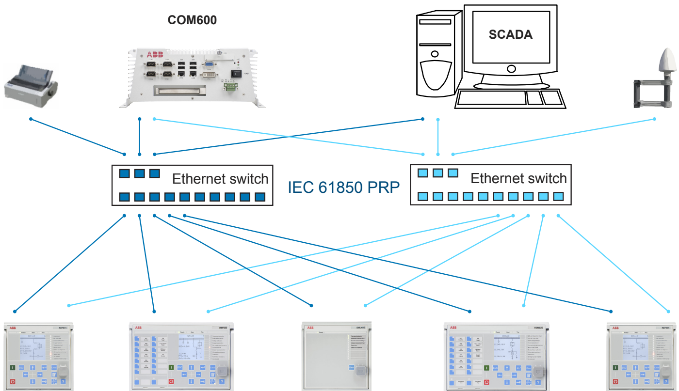
Figure 7. Parallel redundancy protocol (PRP) solution
