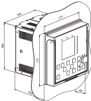
Figure 12. Flush mounting
