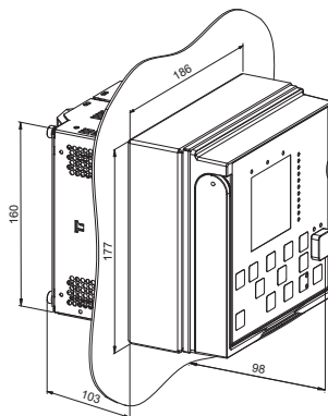
Figure 13. Semi-flush mounting
