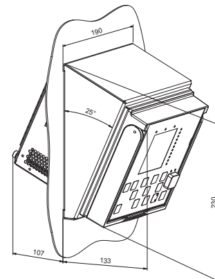
Figure 14. Semi-flush mounting in a 25° tilt
